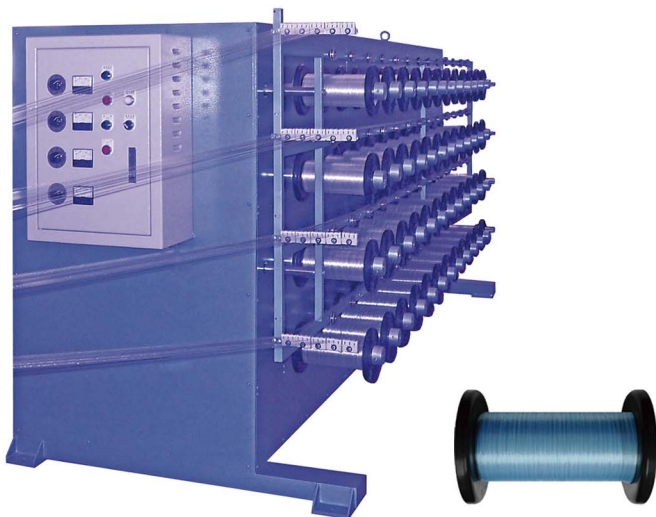
Flange Type Winding Unit
